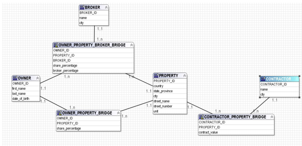
Figure 3. Joining two schemas with a bridge table
