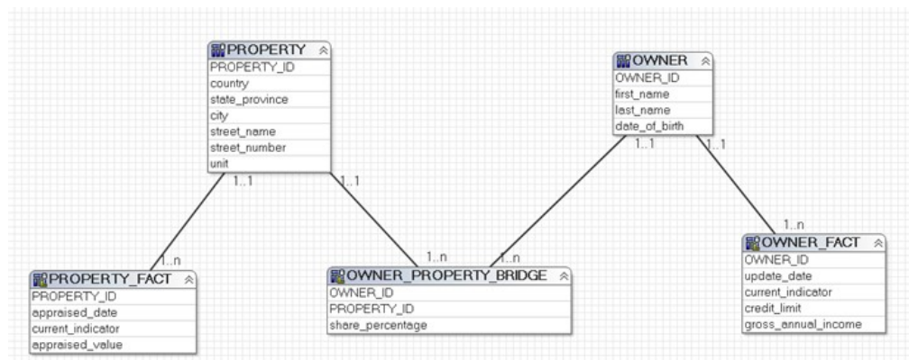
Figure 1. Joining two schemas with a bridge table
