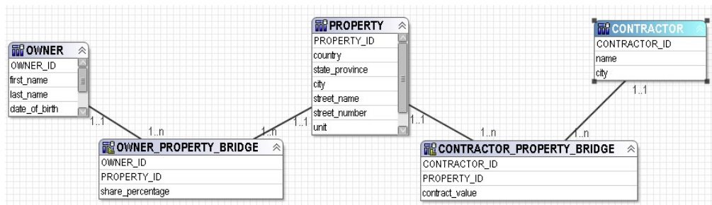
Figure 2. Joining two schemas with multiple bridge table
